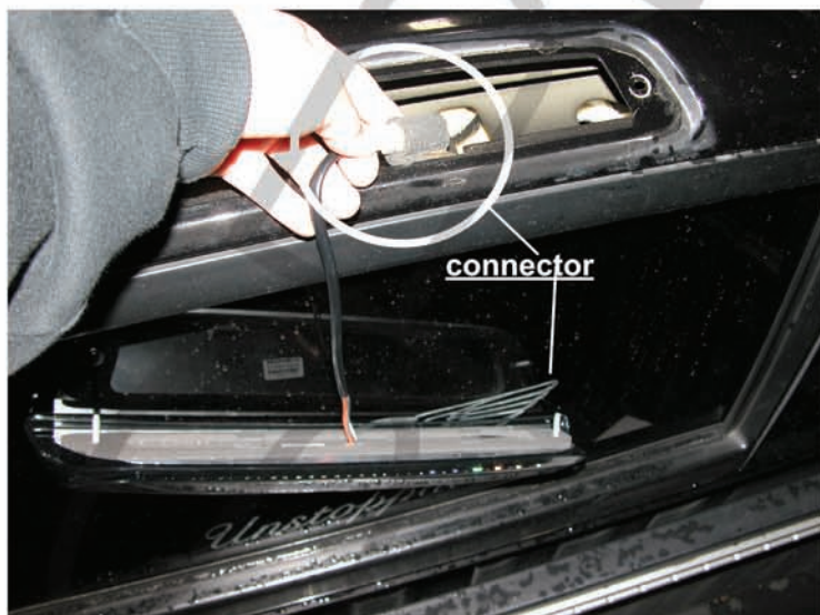
9. Plug the connector harness with the new 3rd brake light
