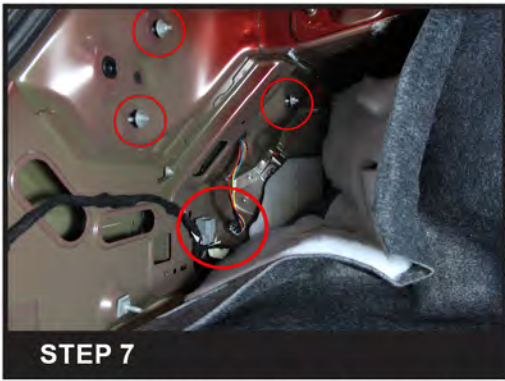
STEP 7 Install the (3) 10mm nuts and connect the taillight connector
