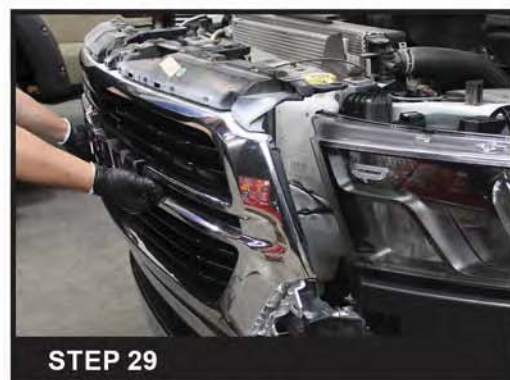
STEP 29 Reinstall the front grille
